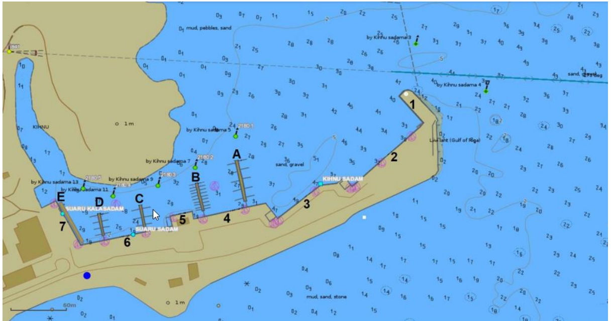
Port layout and Location plan of navigation marks and signs
